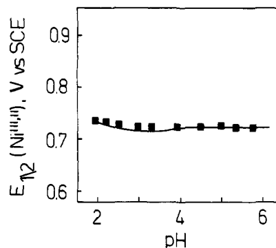
Figure 4. Plot of E_{1/2}(\text{Ni}^{\text{III}}/\text{Ni}^{\text{II}}) vs. pH for complexes of 4 in aqueous solution made 0.1 M in \text{NaClO}_4 . The solid line corresponds to eq 6.
