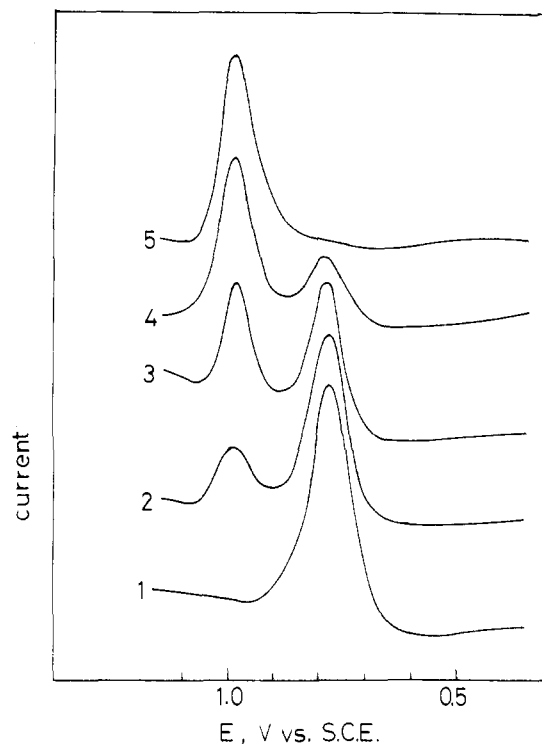
Figure 6. Alternating current voltammetry profiles (oxidation scan) obtained for aqueous solutions of \text{Ni(4)(ClO}_4)_2 of varying concentrations of \text{HClO}_4 : (1) C(\text{HClO}_4) = 1 \times 10^{-2} \text{ M} ; (2) 3 \times 10^{-2} \text{ M} ; (3) 6 \times 10^{-2} \text{ M} ; (4) 1 \times 10^{-1} \text{ M} ; (5) 2 \times 10^{-1} \text{ M} .
