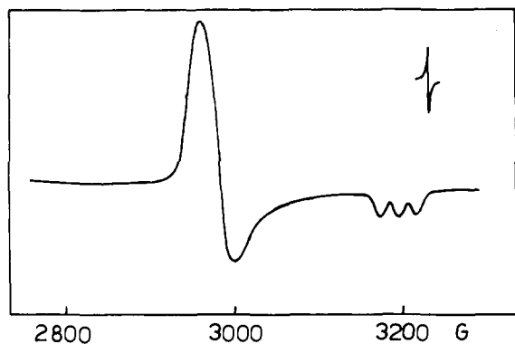
Figure 3. ESR spectrum (recorded at 77 K) of a 1 \times 10^{-3} M solution of \text{Ni(4)}^{3+} in \text{Me}_2\text{SO} (made 0.1 M in \text{Et}_4\text{NBF}_4 ) generated through controlled potential electrolysis. g_{\perp} = 2.16 , g_{\parallel} = 2.03 .
