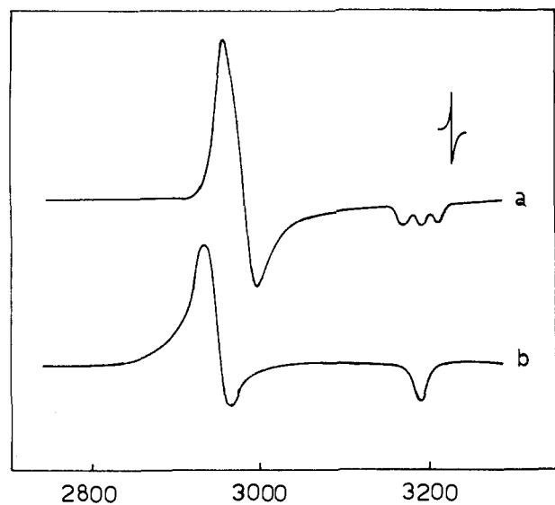
Figure 5. ESR spectrum of aqueous frozen solutions (77 K) of \text{Ni(4)}^{3+} at varying concentrations of \text{HClO}_4 : (a) C(\text{HClO}_4) = 0.01 \text{ M} , the signal is due to the [\text{Ni}^{\text{III}}\text{L}]^{3+} species, g_{\perp} = 2.16 , g_{\parallel} = 2.03 ; (b) C(\text{HClO}_4) = 0.2 \text{ M} , the signal is due to the [\text{Ni}^{\text{III}}\text{LH}]^{4+} species, g_{\perp} = 2.23 , g_{\parallel} = 2.02 ; compare to [\text{Ni}^{\text{III}}(\text{cyclam})]^{3+} values. 15
