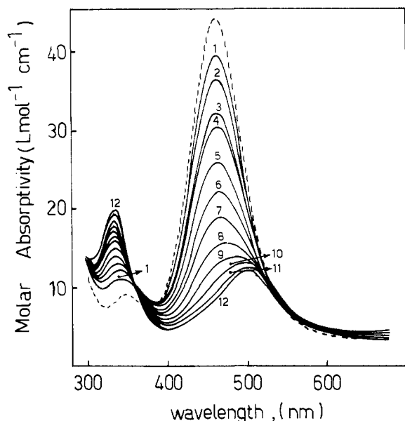
Figure 2. Absorption spectra of a 9 \times 10^{-3} M solution of \text{Ni(4)(ClO}_4)_2 , made 0.1 M in \text{NaClO}_4 , measured at varying pH values: (1) 2.00; (2) 2.20; (3) 2.30; (4) 2.45; (5) 2.65; (6) 2.80; (7) 3.00; (8) 3.20; (9) 3.40; (10) 3.60; (11) 3.60; (12) 4.20. At higher pH values (up to pH 12) the spectrum did not show further changes. The dotted line refers to a solution made 0.1 M in \text{HClO}_4 in which the complex should exist as 100% of the [\text{Ni}^{\text{II}}\text{LH}]^{3+} form.
